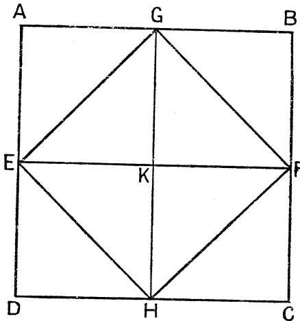
FIG. 4.—EVALUATION OF \sqrt{2} .
